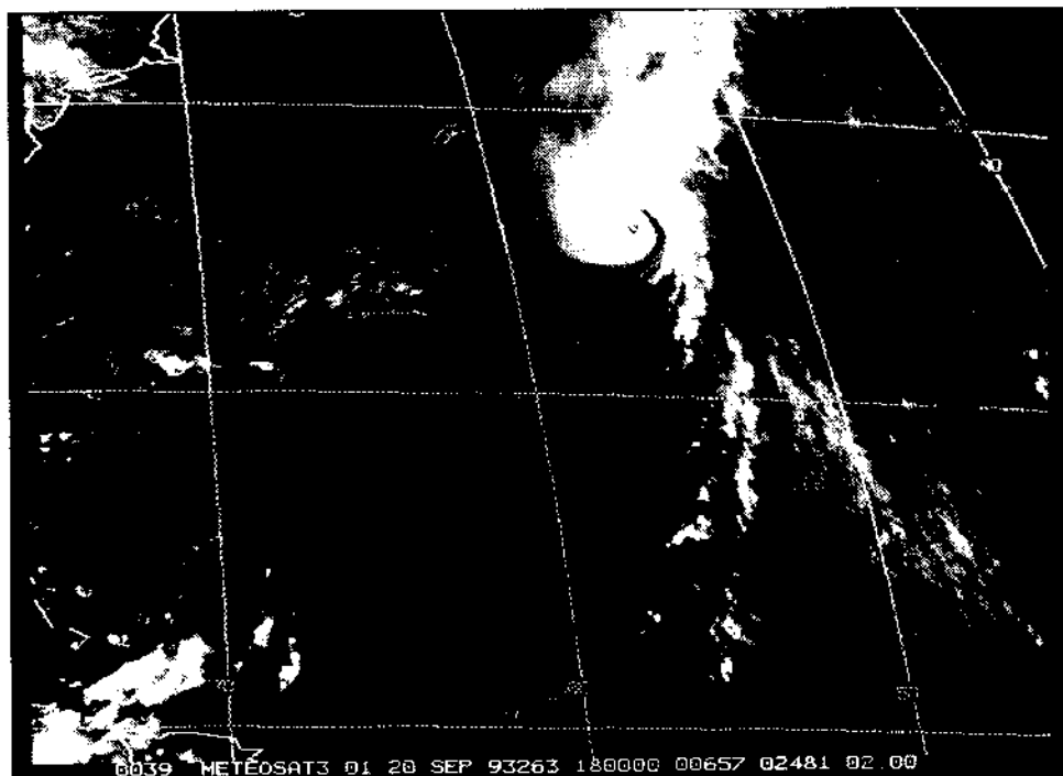
FIG. 7. Meteosat-3 visible satellite image of Hurricane Harvey at 1800 UTC 20 September 1993, showing the appearance of an eye.
