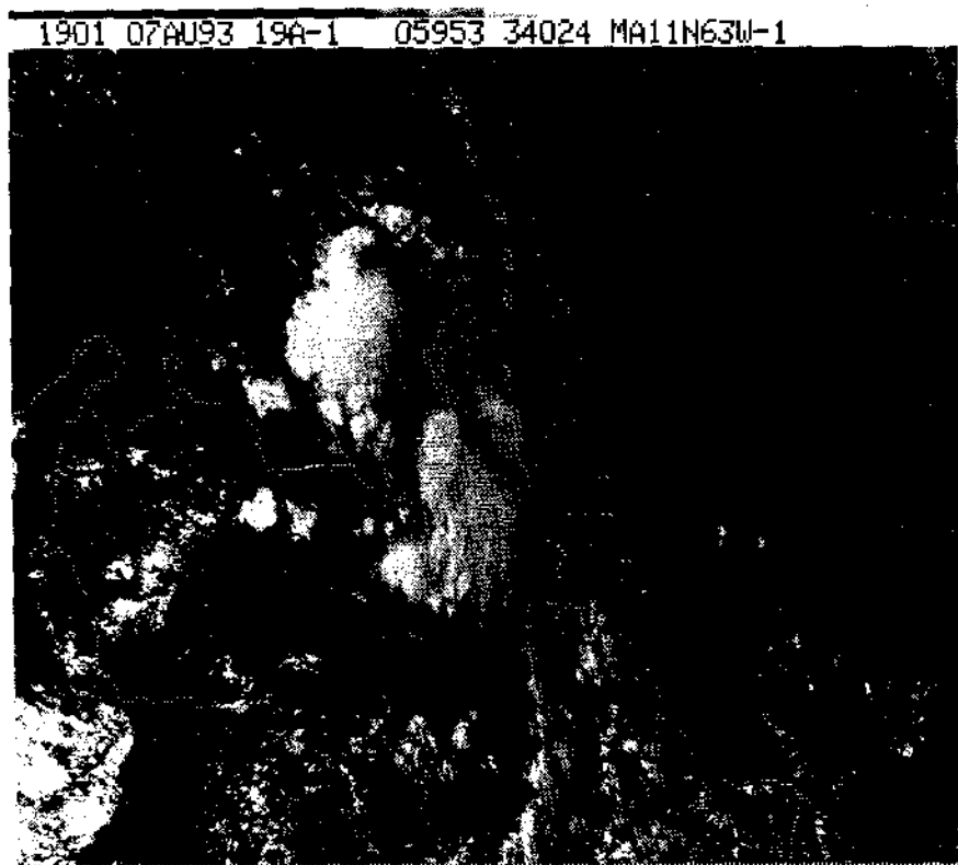
FIG. 3. GOES-7 visible satellite image of Tropical Storm Bret at 1901 UTC 7 August 1993, as heavy rains began spreading over Venezuela.
