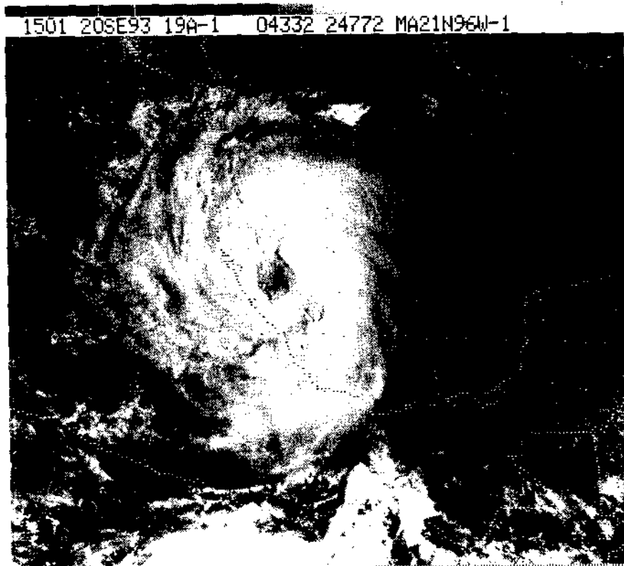
FIG. 6. GOES-7 visible satellite image of Hurricane Gert nearing the coast of Mexico at 1501 UTC 20 September 1993.
