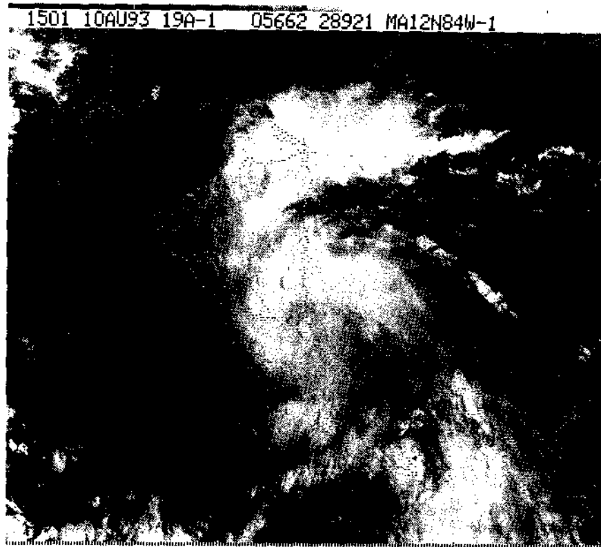
FIG. 4. GOES-7 visible satellite image of rejuvenated Tropical Storm Bret at 1501 UTC 10 August 1993, just prior to landfall over southern Nicaragua.
