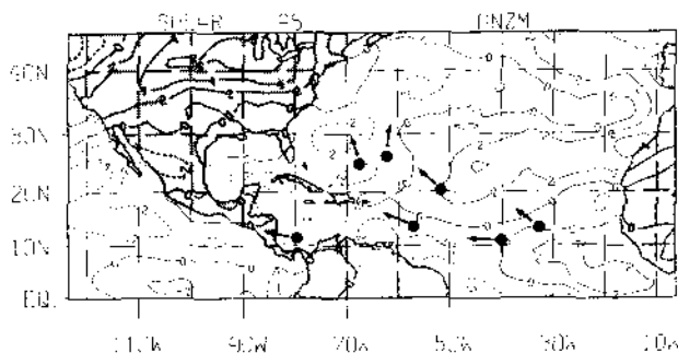
FIG. 2. Anomalies, from the 1975–93 mean, of the magnitude of the vertical shear of the horizontal wind (approximately 900 mb minus 200 mb) for August and September of 1993. Contour interval is 2 \text{ m s}^{-1} with dashed contours for negative anomalies (i.e., weaker than normal shear). Dots show the location where 1993 tropical storms or hurricanes formed (became tropical depressions) in those two months, and arrowheads show direction of motion of the systems during early stages of development.
