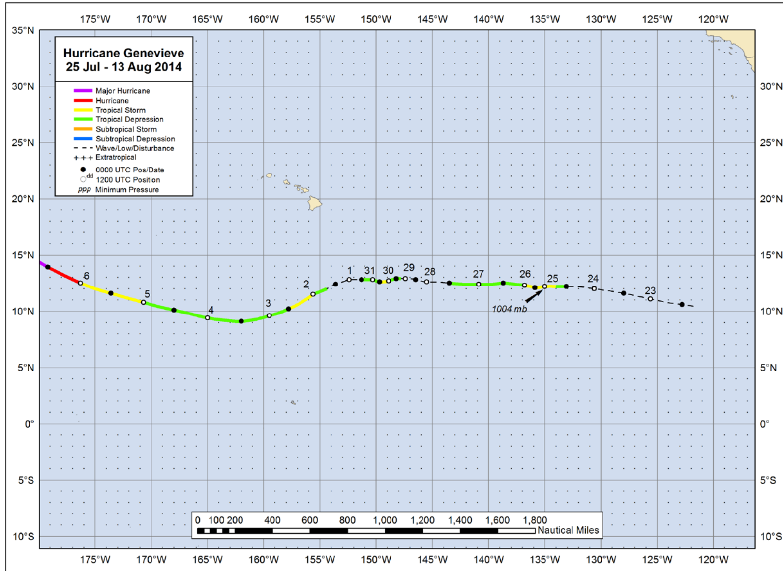
Figure 1. Best track positions for Hurricane Genevieve, 25 July – 13 August, 2014. Best track data west of 140°W longitude was provided by the Central Pacific Hurricane Center and the Joint Typhoon Warning Center.
