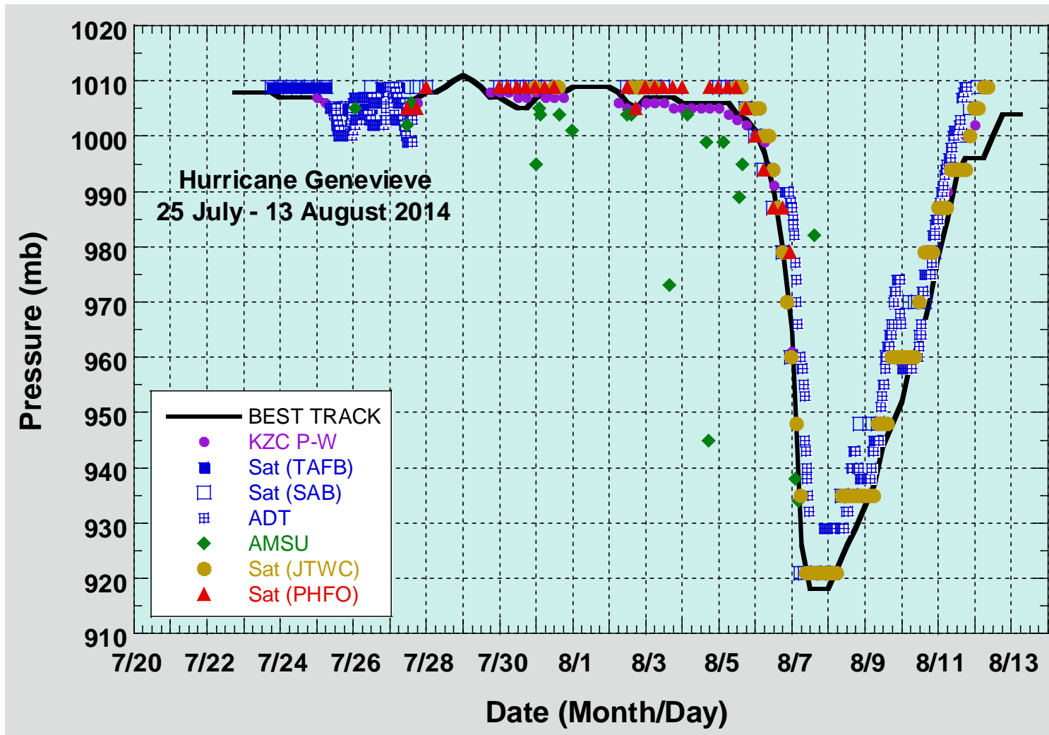
Figure 3. Selected pressure observations and best track minimum central pressure curve for Hurricane Genevieve, 25 – 13 August 2014. Advanced Dvorak Technique estimates represent the Current Intensity at the nominal observation time. AMSU intensity estimates are from the Cooperative Institute for Meteorological Satellite Studies technique. KZC P-W refers to pressure estimates derived using the Knaff-Zehr-Courtney pressure-wind relationship. Dashed vertical lines correspond to 0000 UTC. Best track data west of 140°W longitude was provided by the Central Pacific Hurricane Center and the Joint Typhoon Warning Center.
