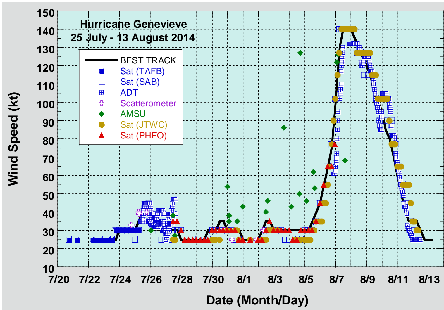
Figure 2. Selected wind observations and best track maximum sustained surface wind speed curve for Hurricane Genevieve, 25 July – 13 August 2014. Advanced Dvorak Technique estimates represent the Current Intensity at the nominal observation time. AMSU intensity estimates are from the Cooperative Institute for Meteorological Satellite Studies technique. Dashed vertical lines correspond to 0000 UTC. Best track data west of 140°W longitude was provided by the Central Pacific Hurricane Center and the Joint Typhoon Warning Center.
