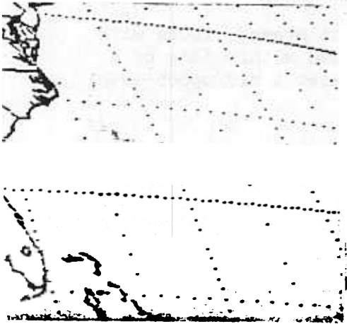
Visible (VIS = 0.65um)
