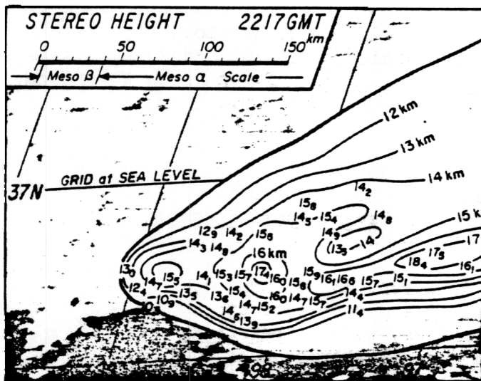
Fig.8 LEFT: Stereo height (in km) superimposed upon the visible imagery at 2217GMT 2 May 1979. RIGHT: IR isotherms (in °C) superimposed upon the enhanced IR imagery at the same time. These pictures reveal that the IR temperatures are warm and stereo heights are high inside the horseshoe wake. On the upwind side of the wake, however, the higher the stereo height, the colder the IR temperature.
