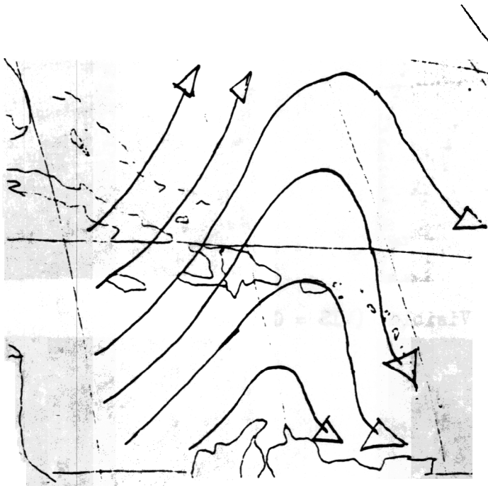
200mb Streamlines
