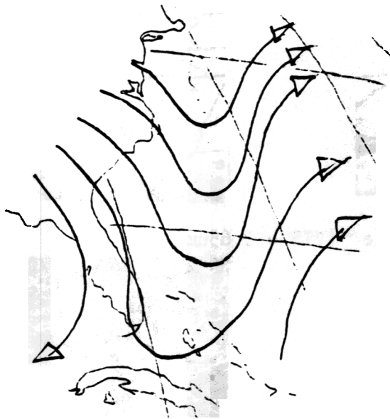
500mb Streamlines
