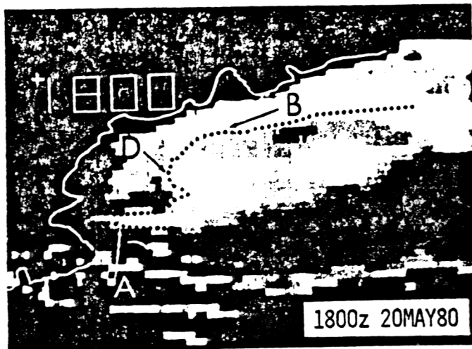
Fig. 16. GOES-East IR 20 May 1980, 1800 GMT.
