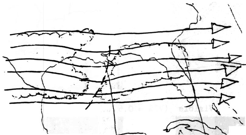
200mb Streamlines
