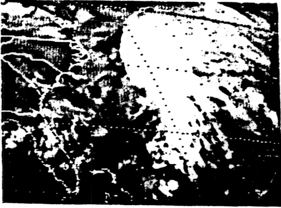
Infrared (IR = 11 um)
