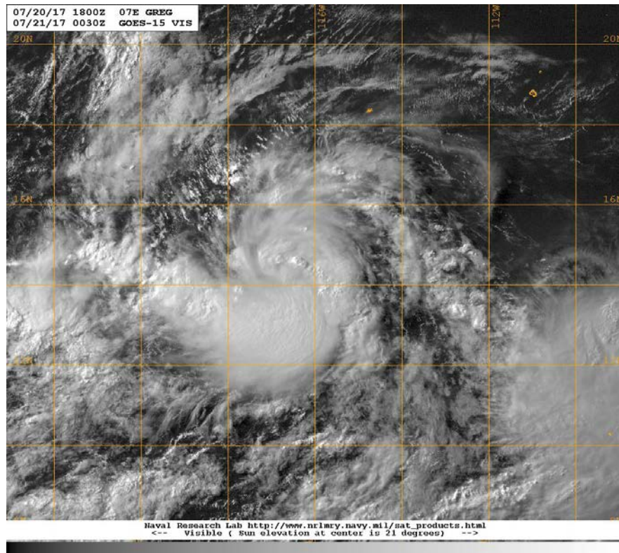
GOES-15 VISIBLE SATELLITE IMAGE OF TROPICAL STORM GREG NEAR ITS ESTIMATED MAXIMUM INTENSITY OF 50 KT AT 0030 UTC 21 JULY 2017. IMAGE COURTESY OF NAVAL RESEARCH LABORATORY.
