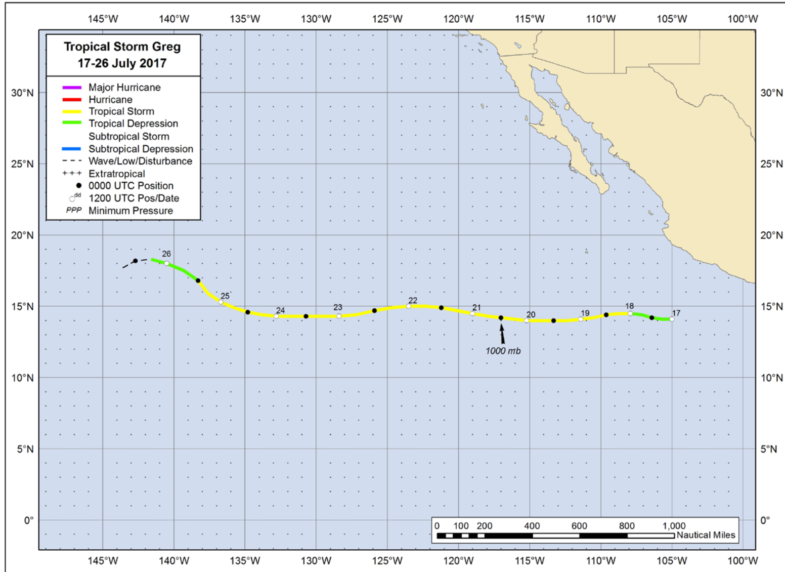
Figure 1. Best track positions for Tropical Storm Greg, 17–26 July 2017.
