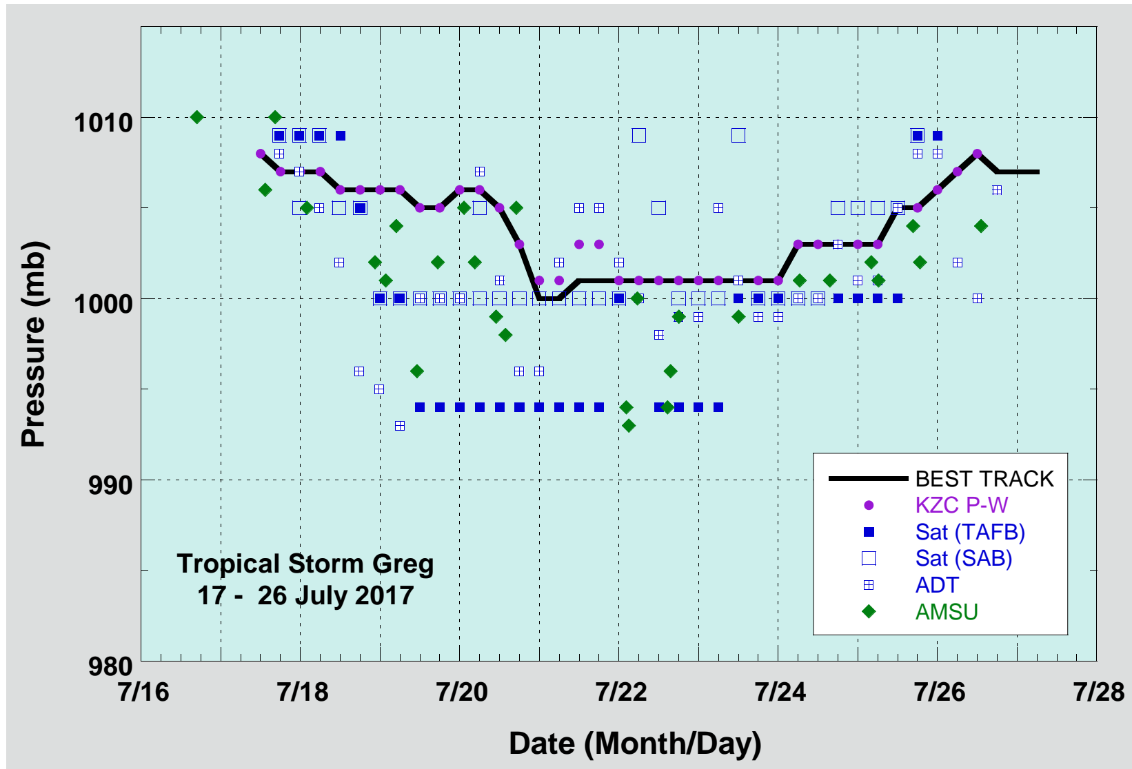
Figure 3. Selected pressure observations and best track minimum central pressure curve for Tropical Storm Greg, 17–26 July 2017. Advanced Dvorak Technique estimates represent the Current Intensity at the nominal observation time. AMSU intensity estimates are from the Cooperative Institute for Meteorological Satellite Studies technique. KZC P-W refers to pressure estimates derived using the Knaff-Zehr-Courtney pressure-wind relationship. Dashed vertical lines correspond to 0000 UTC.
