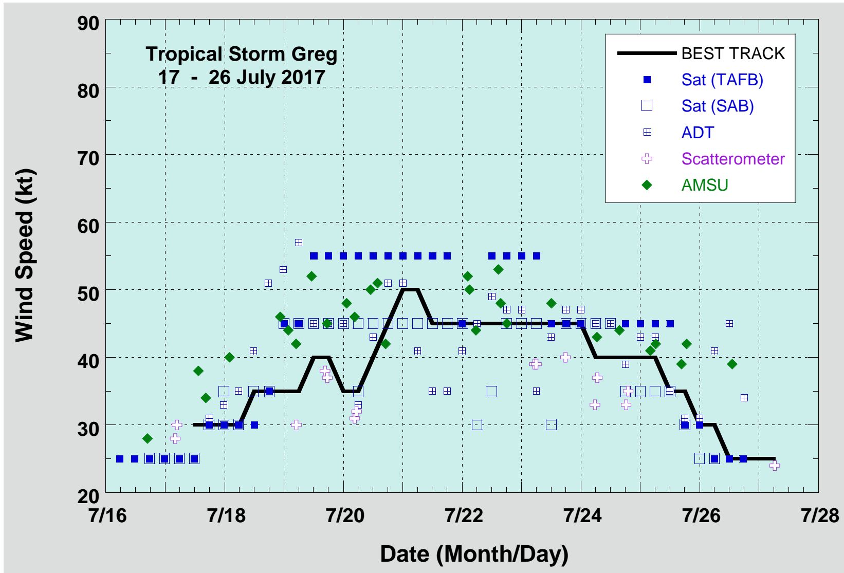
Figure 2. Selected wind observations and best track maximum sustained surface wind speed curve for Tropical Storm Greg, 17–26 July 2017. Advanced Dvorak Technique estimates represent the Current Intensity at the nominal observation time. AMSU intensity estimates are from the Cooperative Institute for Meteorological Satellite Studies technique. Dashed vertical lines correspond to 0000 UTC.
