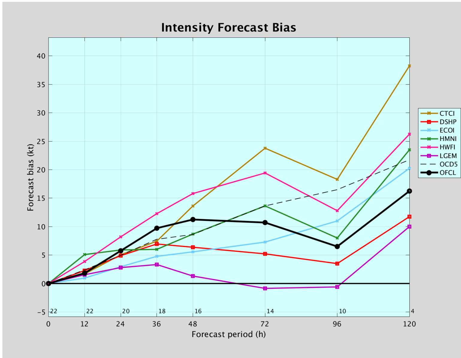
Figure 4. Selected model forecast intensity bias for Tropical Storm Greg, 17–26 July 2017. The statistical-dynamical models (DSHP and LGEM) had generally less bias and lower absolute error than the global or hurricane dynamical models.
